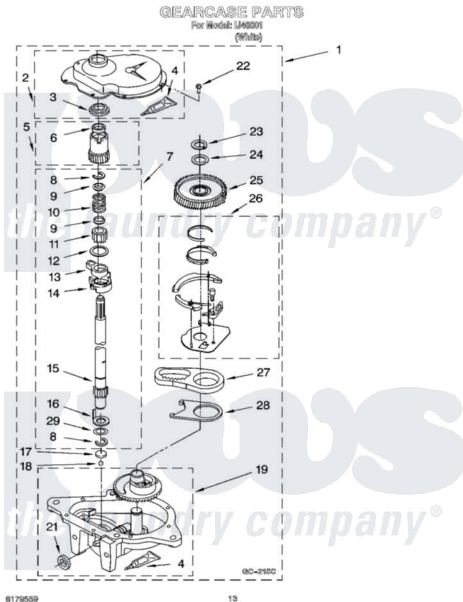
Whirlpool Residential Whirlpool IJ46001 Washer Parts Parts Diagram 09 - GEARCASE PARTS Click on the part number to view part
