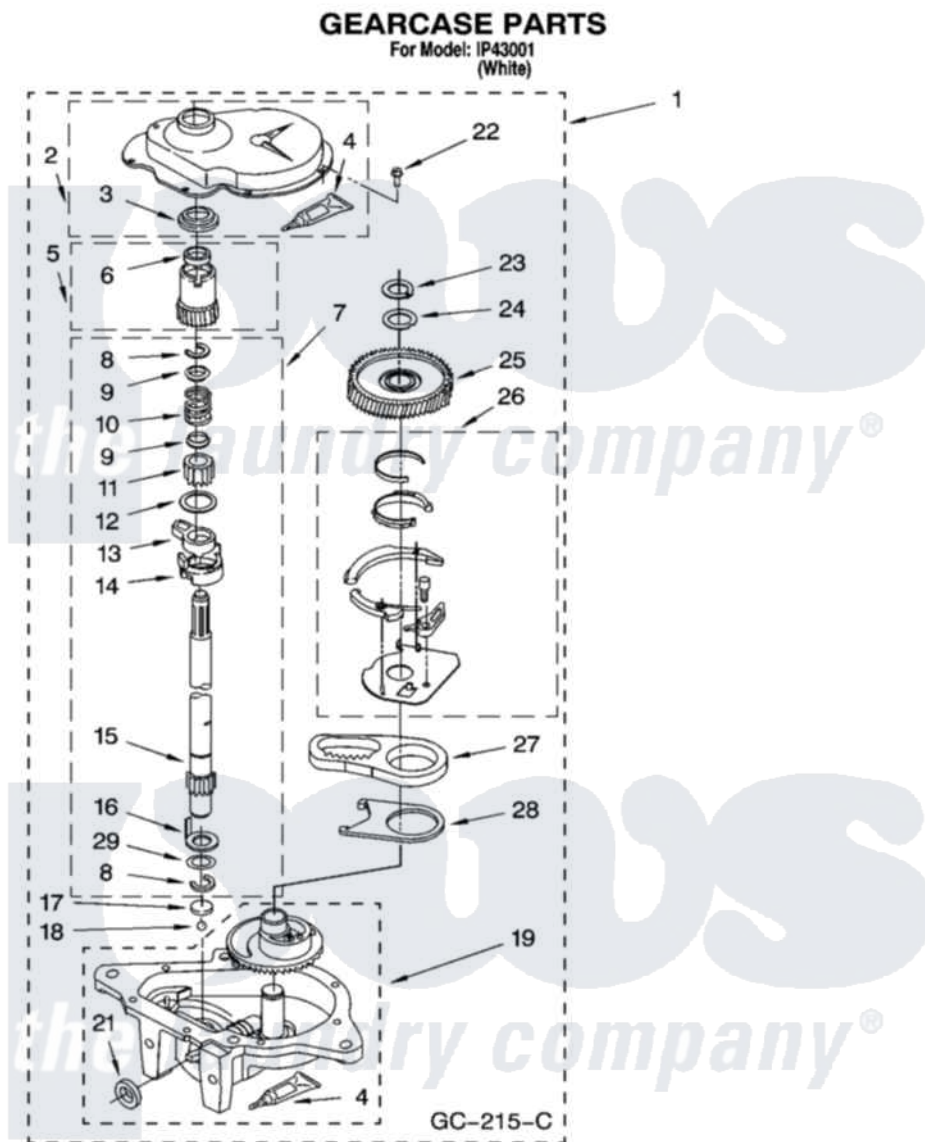
Whirlpool Residential Whirlpool IP43001 Washer Parts Parts Diagram 08 - GEARCASE PARTS Click on the part number to view part
