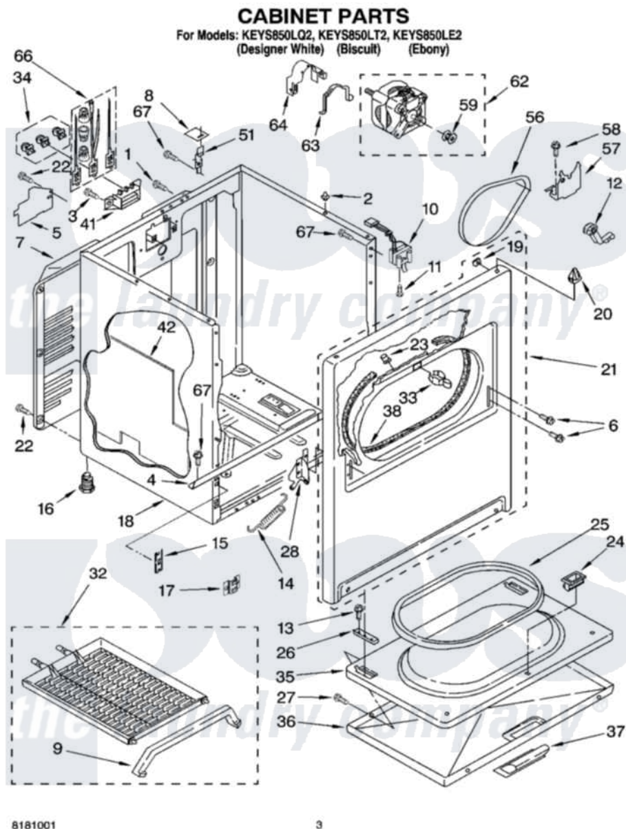
Whirlpool Residential Whirlpool KEYS850LQ2 Dryer Parts Parts Diagram 02 - CABINET PARTS
