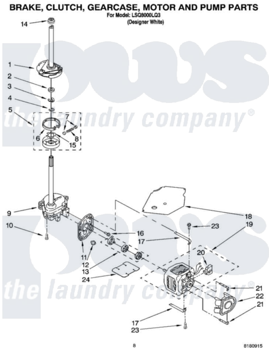
Whirlpool Residential Whirlpool LSQ8000LQ3 Washer Parts Parts Diagram 05 - BRAKE, CLUTCH, GEARCASE, MOTOR AND PUMP PARTS Click on the part number to view part
