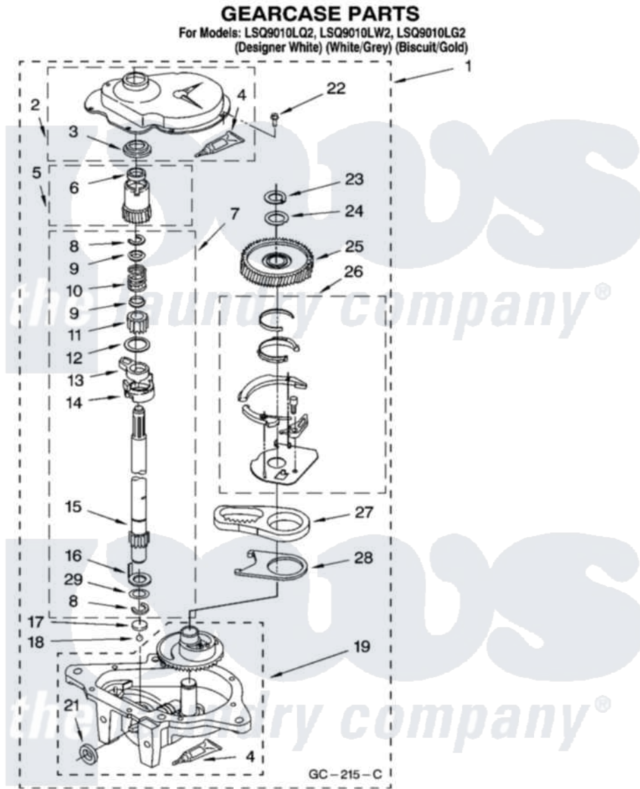
Whirlpool Residential Whirlpool LSQ9010LW2 Washer Parts Parts Diagram 08 - GEARCASE PARTS Click on the part number to view part
