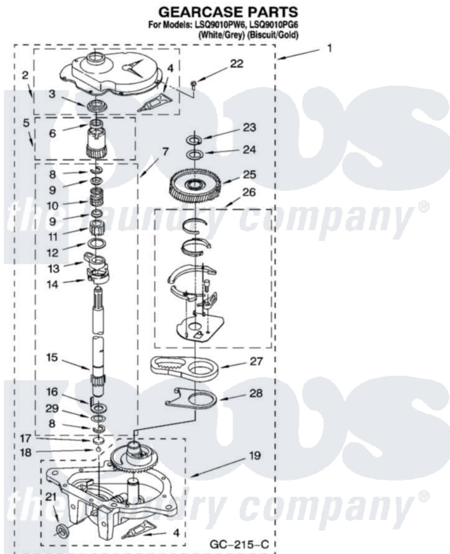
Whirlpool Residential Whirlpool LSQ9010PG6 Washer Parts Parts Diagram 08 - GEARCASE PARTS Click on the part number to view part
