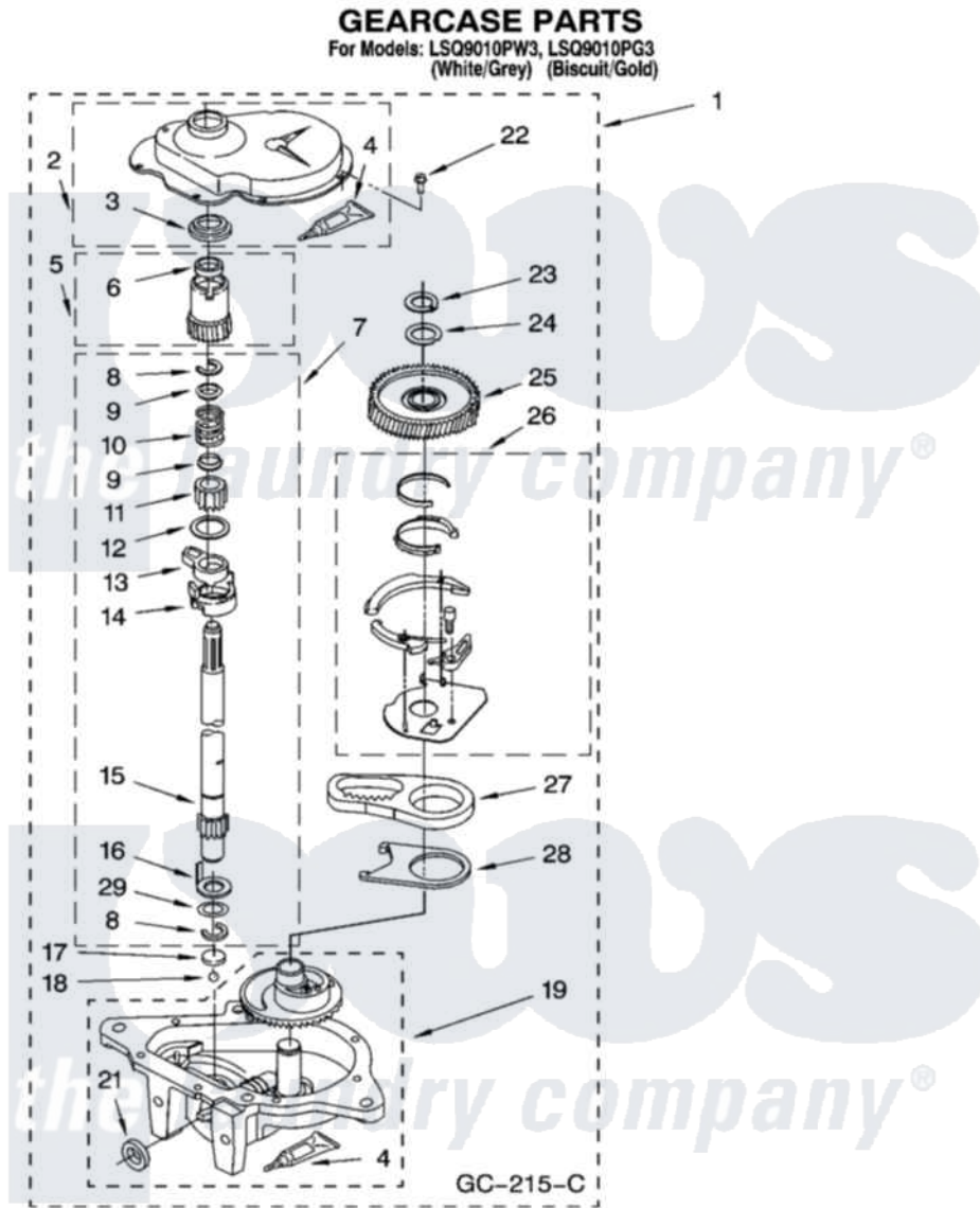
Whirlpool Residential Whirlpool LSQ9010PW3 Washer Parts Parts Diagram 08 - GEARCASE PARTS Click on the part number to view part
