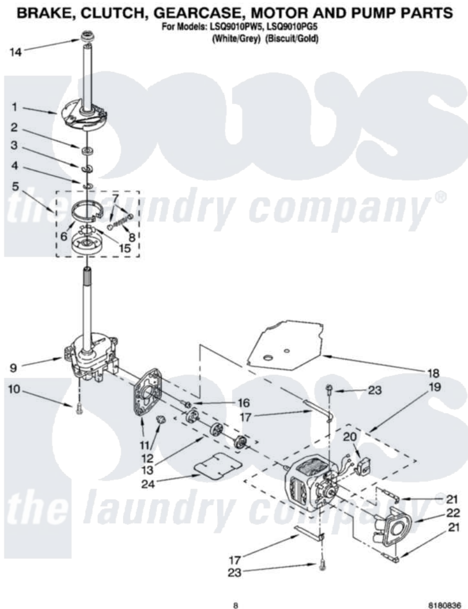
Whirlpool Residential Whirlpool LSQ9010PW5 Washer Parts Parts Diagram 05 - BRAKE, CLUTCH, GEARCASE, MOTOR AND PUMP PARTS Click on the part number to view part
