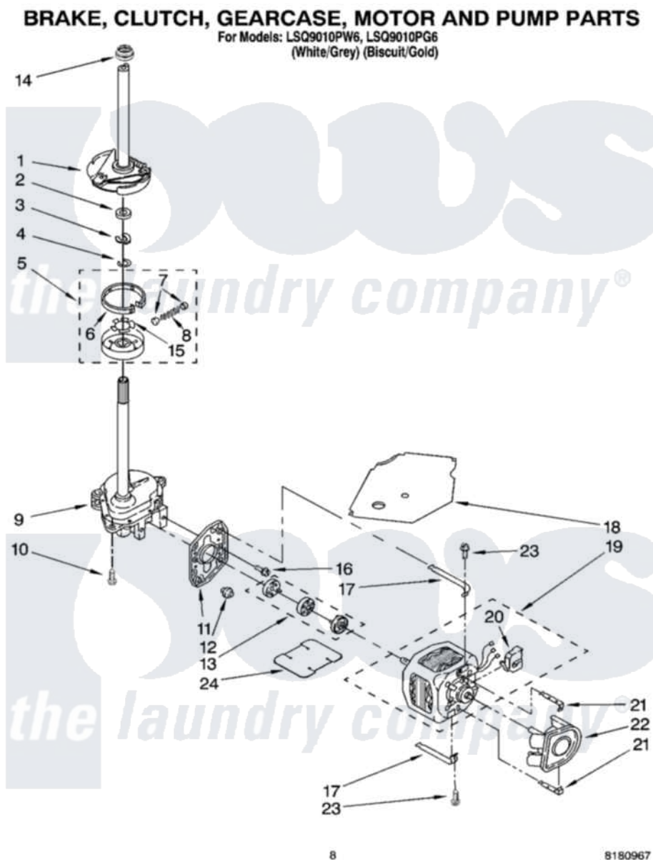
Whirlpool Residential Whirlpool LSQ9010PW6 Washer Parts Parts Diagram 05 - BRAKE, CLUTCH, GEARCASE, MOTOR AND PUMP PARTS Click on the part number to view part
