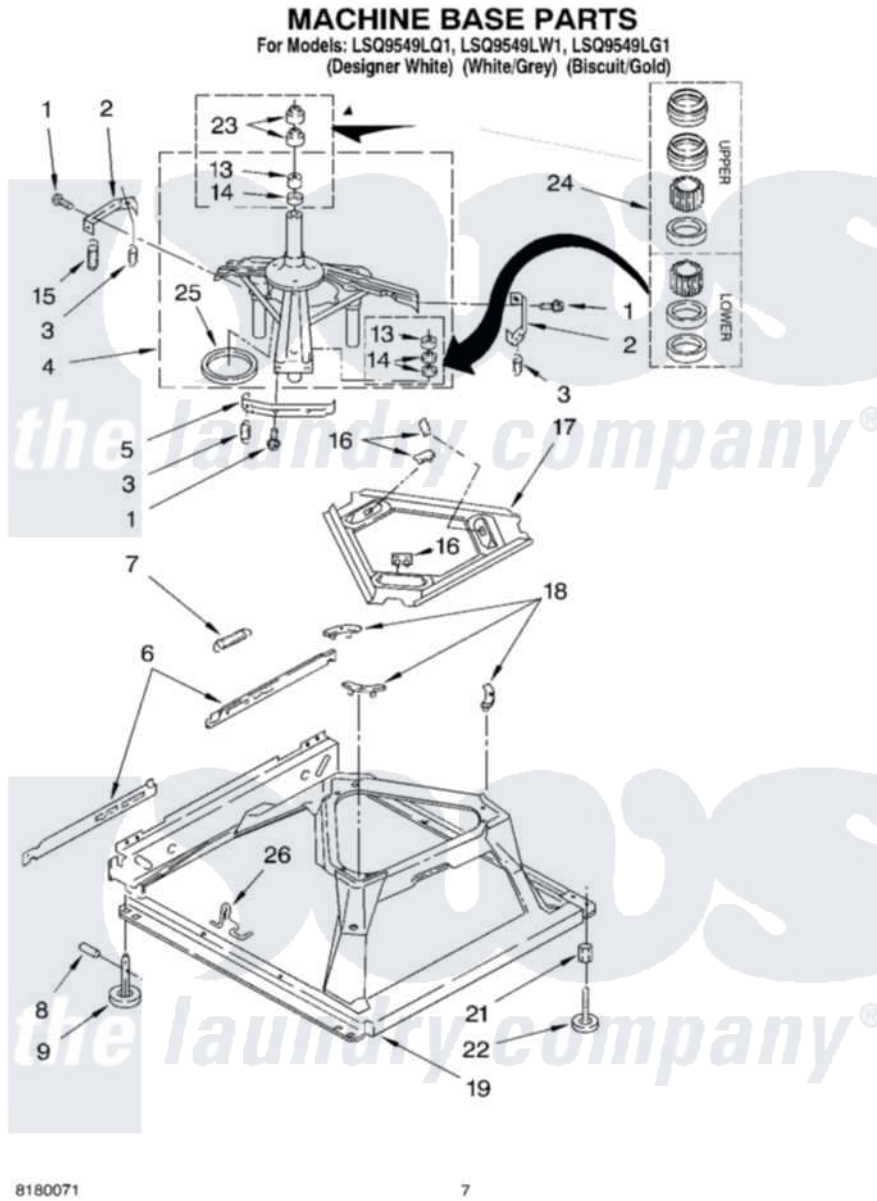
Whirlpool Residential Whirlpool LSQ9549LW1 Washer Parts Parts Diagram 04 - MACHINE BASE PARTS Click on the part number to view part
