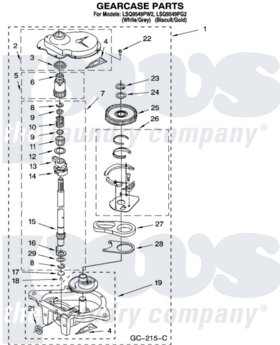
Whirlpool Residential Whirlpool LSQ9549PW2 Washer Parts Parts Diagram 08 - GEARCASE PARTS Click on the part number to view part
