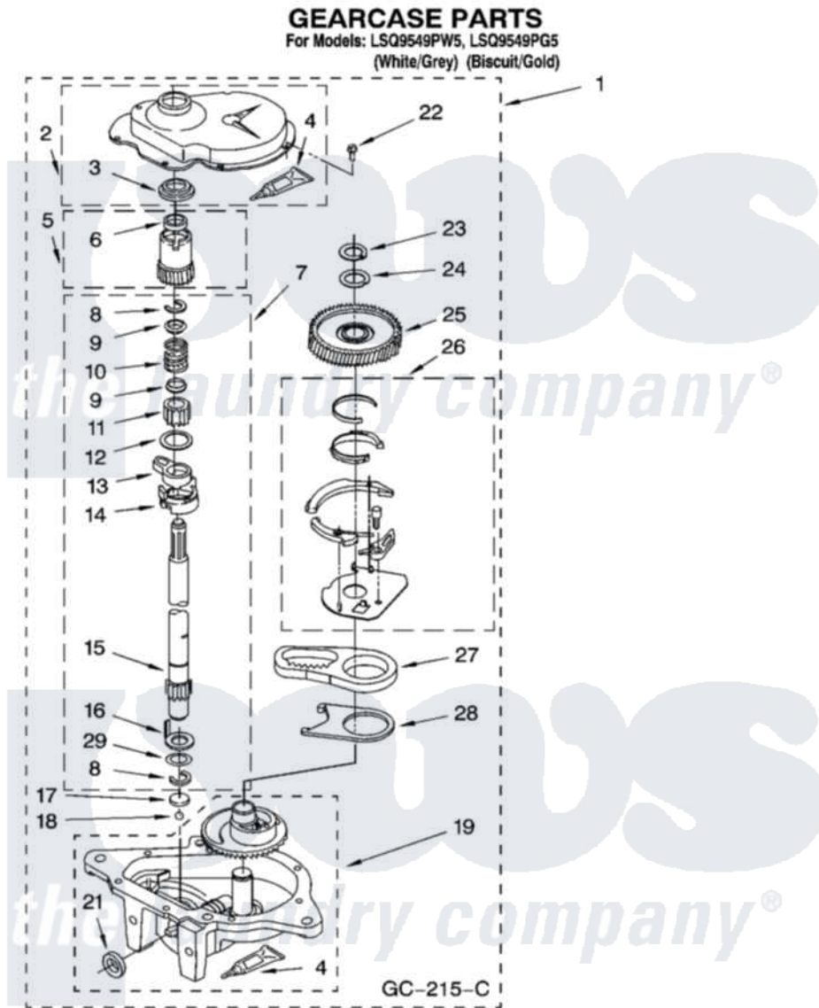
Whirlpool Residential Whirlpool LSQ9549PW5 Washer Parts Parts Diagram 08 - GEARCASE PARTS Click on the part number to view part
