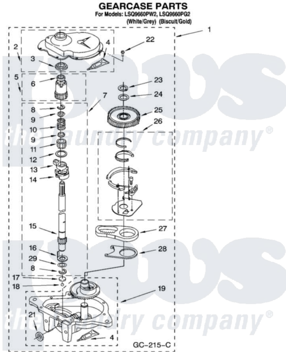
Whirlpool Residential Whirlpool LSQ9660PG2 Washer Parts Parts Diagram 08 - GEARCASE PARTS Click on the part number to view part
