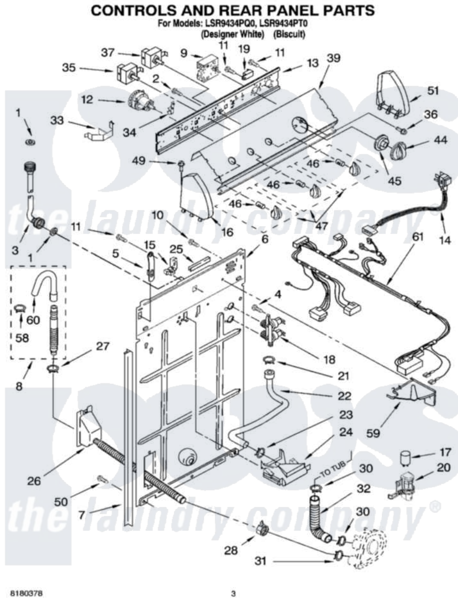
Whirlpool Residential Whirlpool LSR9434PQ0 Washer Parts Parts Diagram 02 - CONTROLS AND REAR PANEL PARTS Click on the part number to view part
