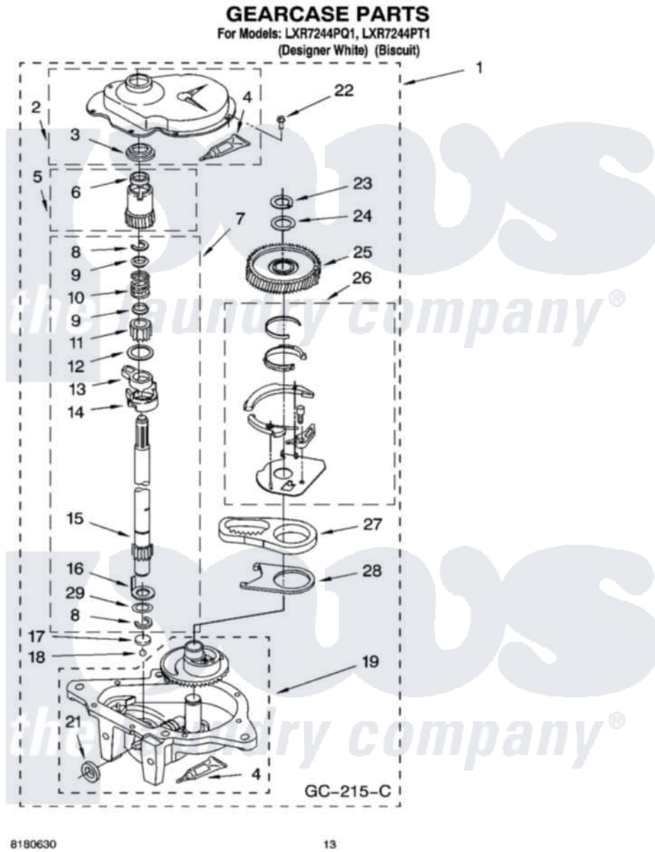
Whirlpool Residential Whirlpool LXR7244PT1 Washer Parts Parts Diagram 09 - GEARCASE PARTS Click on the part number to view part
