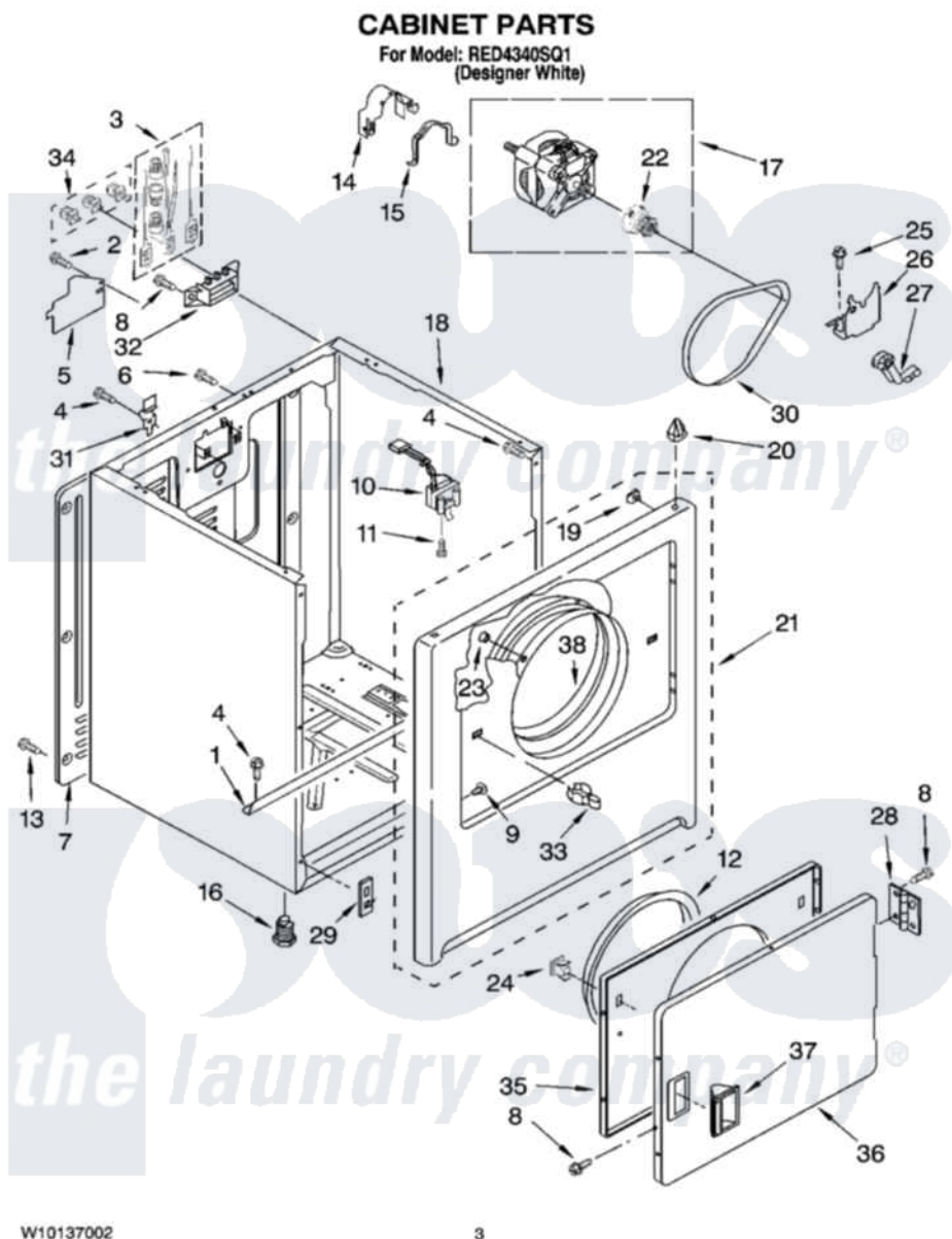
Whirlpool Residential Whirlpool RED4340SQ1 Dryer Parts Parts Diagram 02 - CABINET PARTS Click on the part number to view part
