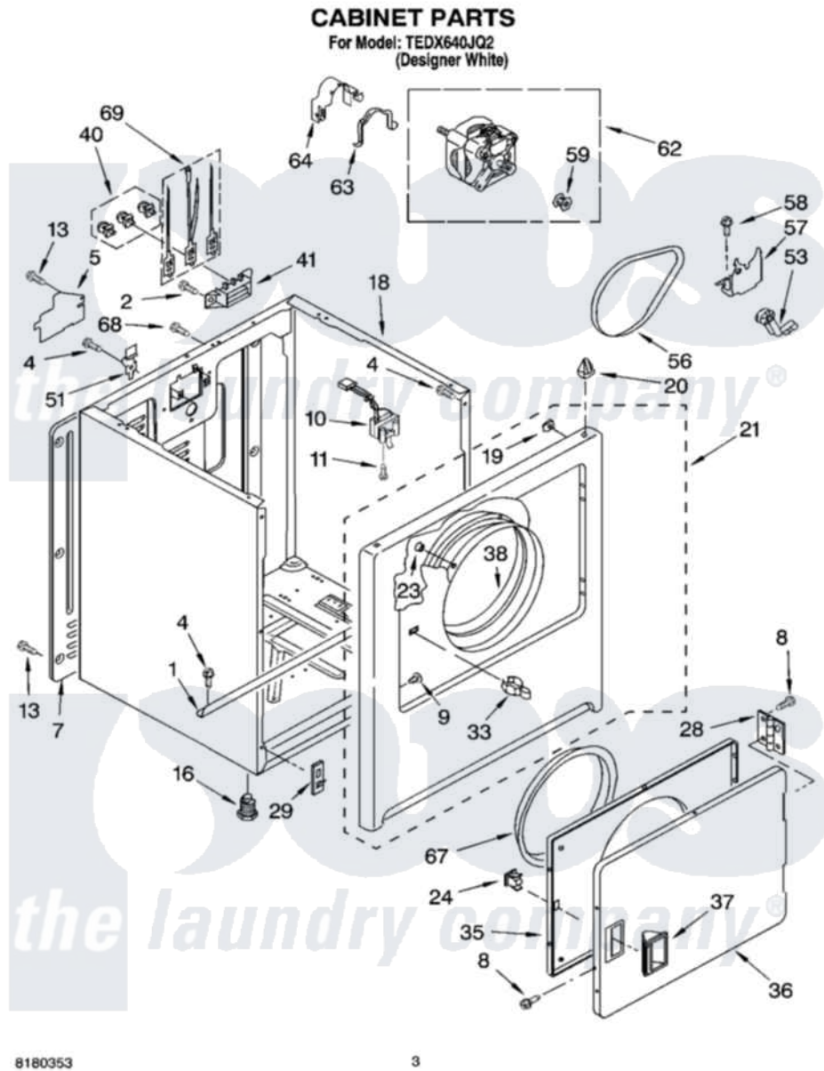
Whirlpool Residential Whirlpool TEDX640JQ2 Dryer Parts Parts Diagram 02 - CABINET PARTS Click on the part number to view part
