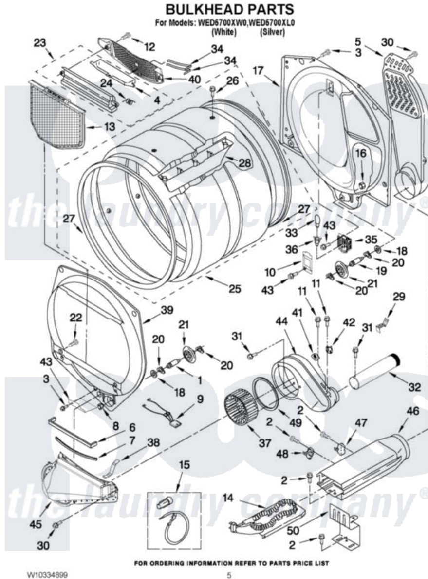
Whirlpool Residential Whirlpool WED5700XL0 Dryer Parts Parts Diagram 03 - BULKHEAD PARTS Click on the part number to view part
