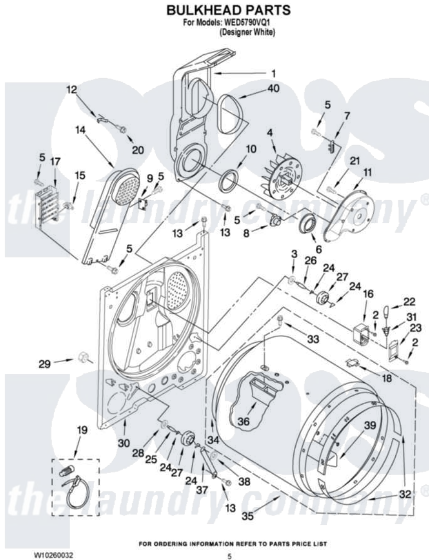
Whirlpool Residential Whirlpool WED5790VQ1 Dryer Parts Parts Diagram 03 - BULKHEAD PARTS Click on the part number to view part
