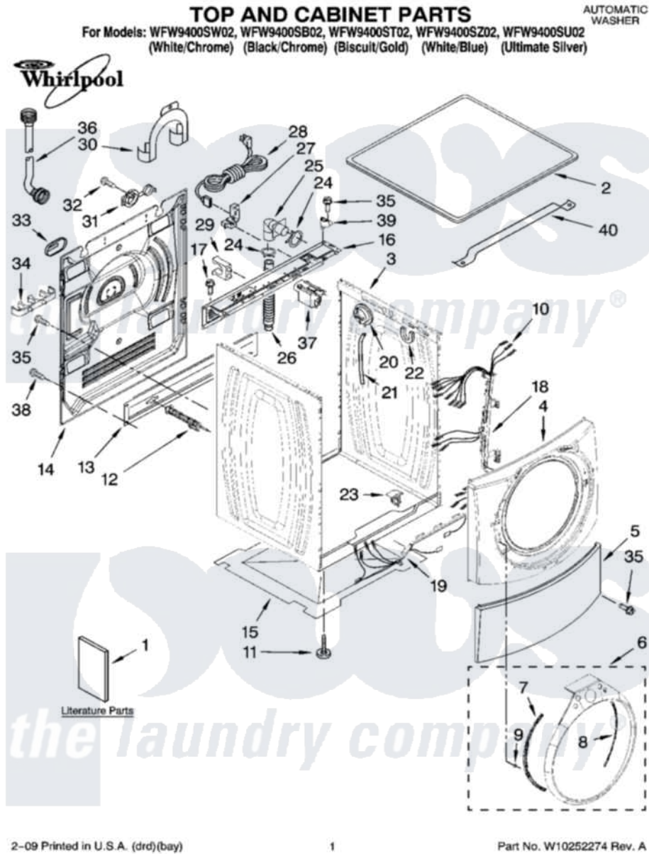
Whirlpool Residential Whirlpool WFW9400ST02 Washer Parts Parts Diagram 01 - TOP AND CABINET PARTS Click on the part number to view part
