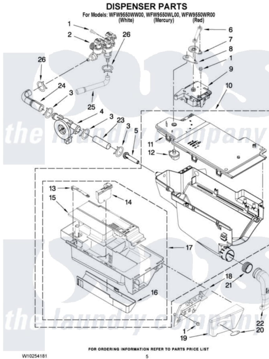
Whirlpool Residential Whirlpool WFW9550WW00 Washer Parts Parts Diagram 04 - DISPENSER PARTS Click on the part number to view part
