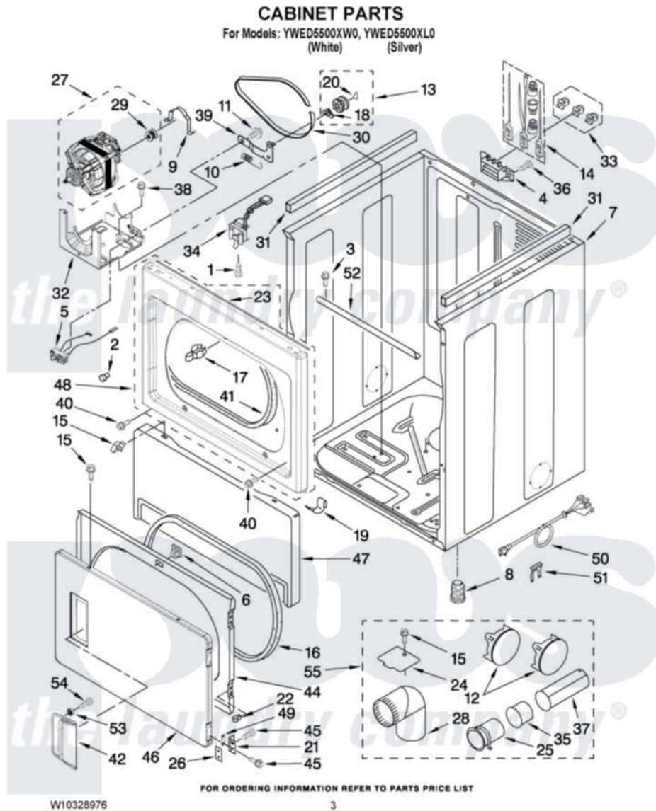
Whirlpool Residential Whirlpool YWED5500XL0 Dryer Parts Parts Diagram 02 - CABINET PARTS Click on the part number to view part
