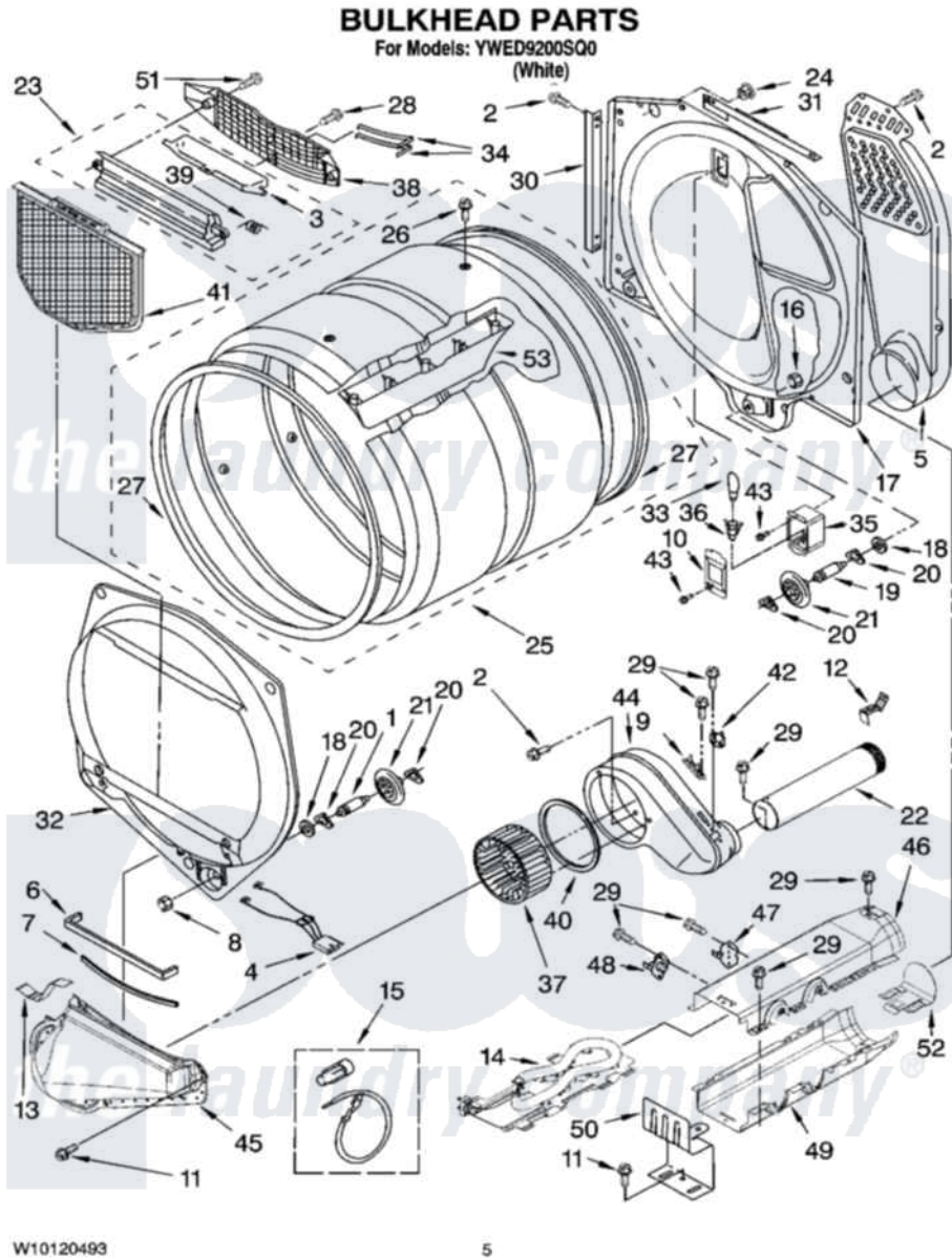
Whirlpool Residential Whirlpool YWED9200SQ0 Dryer Parts Parts Diagram 03 - BULKHEAD PARTS Click on the part number to view part
