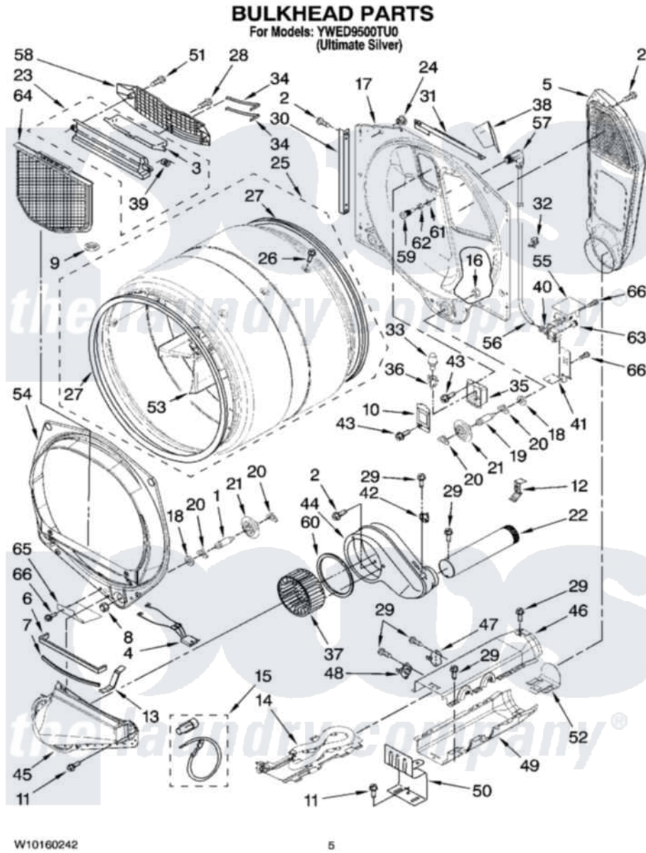
Whirlpool Residential Whirlpool YWED9500TU0 Dryer Parts Parts Diagram 03 - BULKHEAD PARTS Click on the part number to view part
