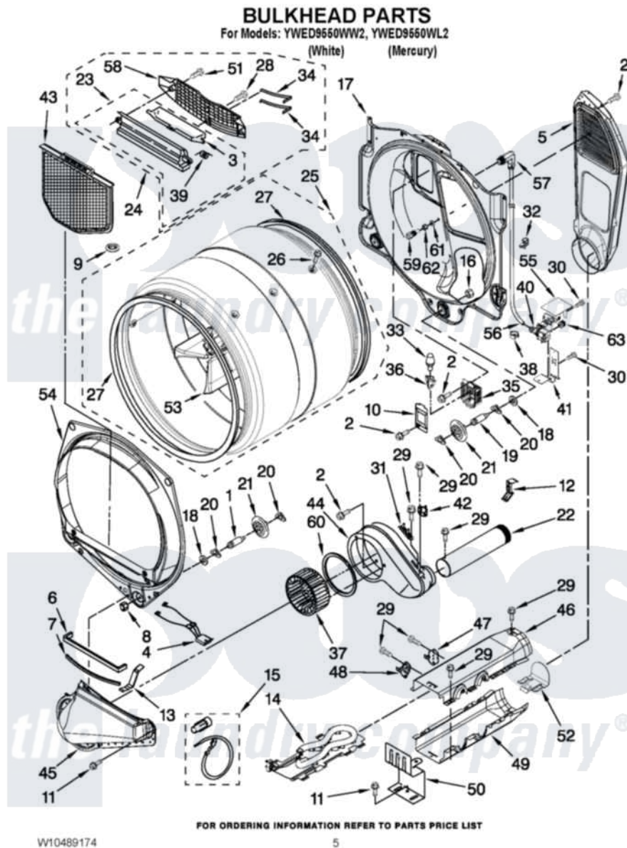
Whirlpool Residential Whirlpool YWED9550WL2 Dryer Parts Parts Diagram 03 - BULKHEAD PARTS Click on the part number to view part
